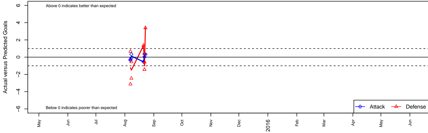
Redmond Team USA B03 Dots are actual minus expected GF (blue circles) and GA (red triangles). Blue line is smoothed change in attack strength. Red is smoothed change in defense strength.
